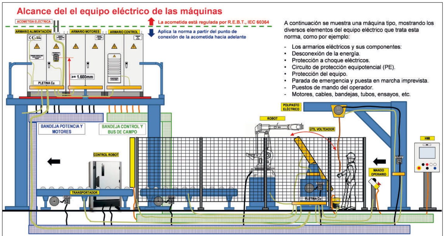
Example of electrical equipment of a machine
