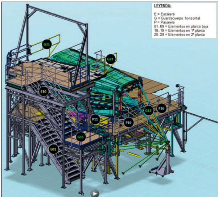
Example of permanent means of access to machinery
