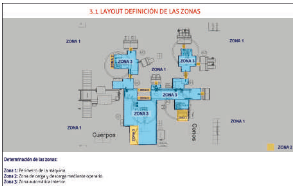
Risk assessment, zones of the machine
