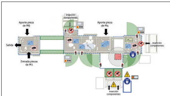
Safety layout
